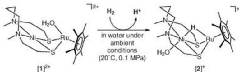
Fig. 2. Formation of a Ni( \mu -H)Ru complex obtained from the reaction of a NiRu aqua complex with dihydrogen ( H_2 ) in water under ambient conditions (20°C and 0.1 MPa).
